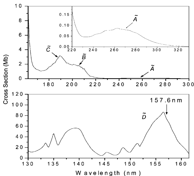
Figure 1. Absorption spectrum of HN 3 at room temperature (adapted from refs 3 and 4). The position of the photolysis excitation wavelength in this work is indicated by arrows (1 Mb = 1 × 10 -18 cm 2 ).
