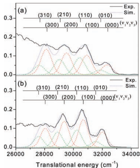
Figure 5. Experimentally derived internal energy profiles together with simulations including progressions in the (\nu_1,00) and (\nu_1,10) modes. The detector direction is (a) perpendicular and (b) parallel to the photolysis laser polarization.
